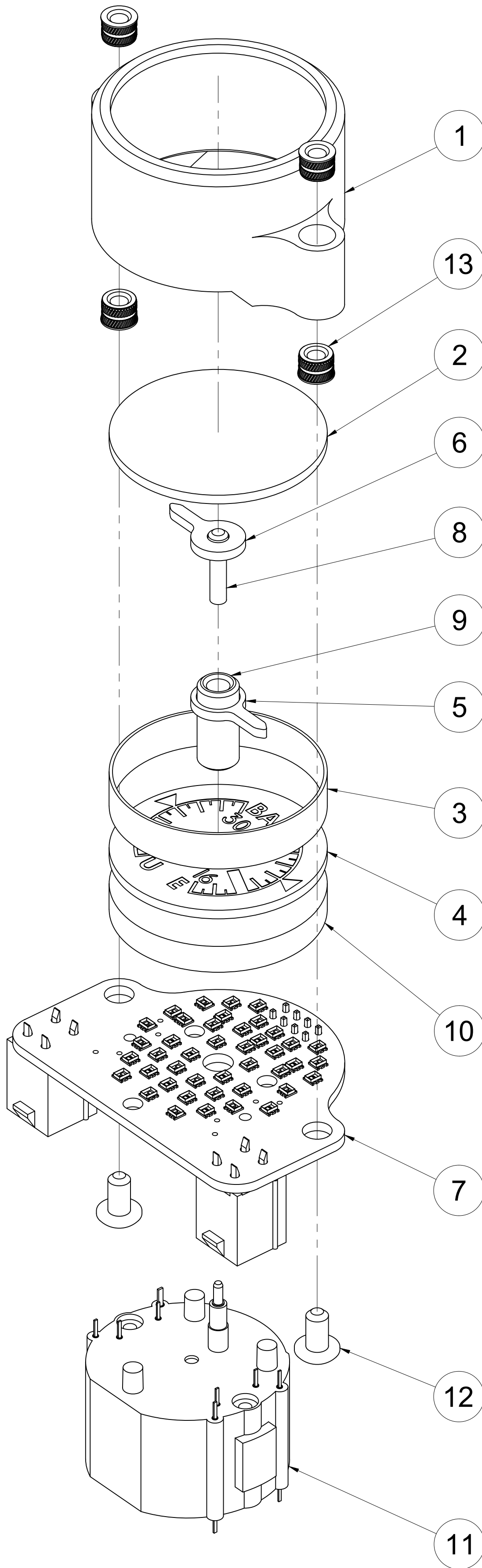
-100 ASSY SCALE 2:1
